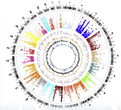
-omic sequencing
