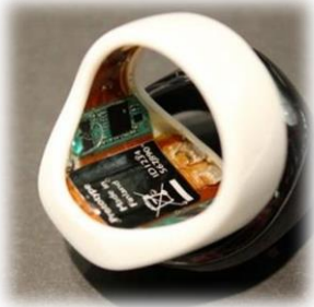
Smart Ring
