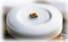
Smart Computer
